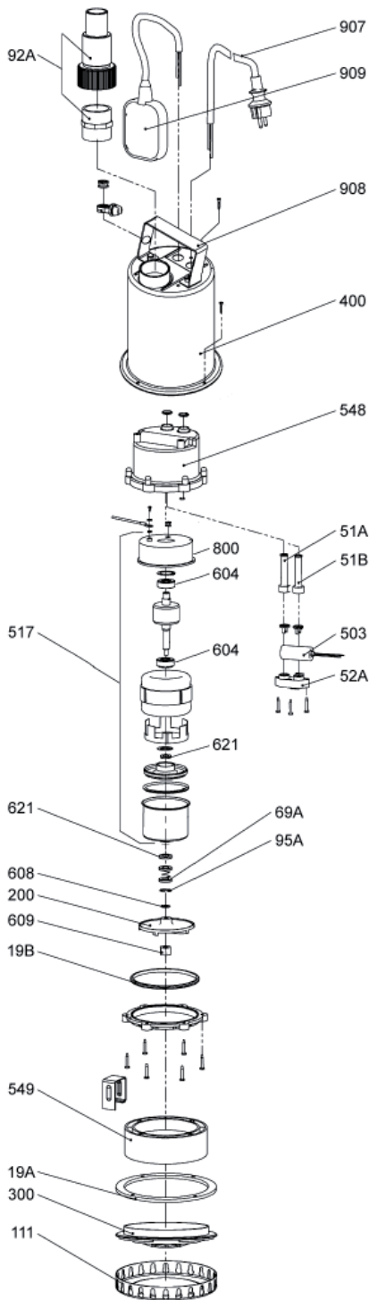
SX-50 (c.9210)
